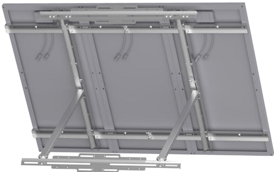
UNIFIX 300 Pour Unisun 80.12M (x3)/ 100.12M (x3)/ 120.12BC (x3)/ 100.24M (x3)/ 150.24M (x2)/ 150.12BC (x2)/ 200.12BC (x2)/ 200.24M/ 300.12M Ref 0378
